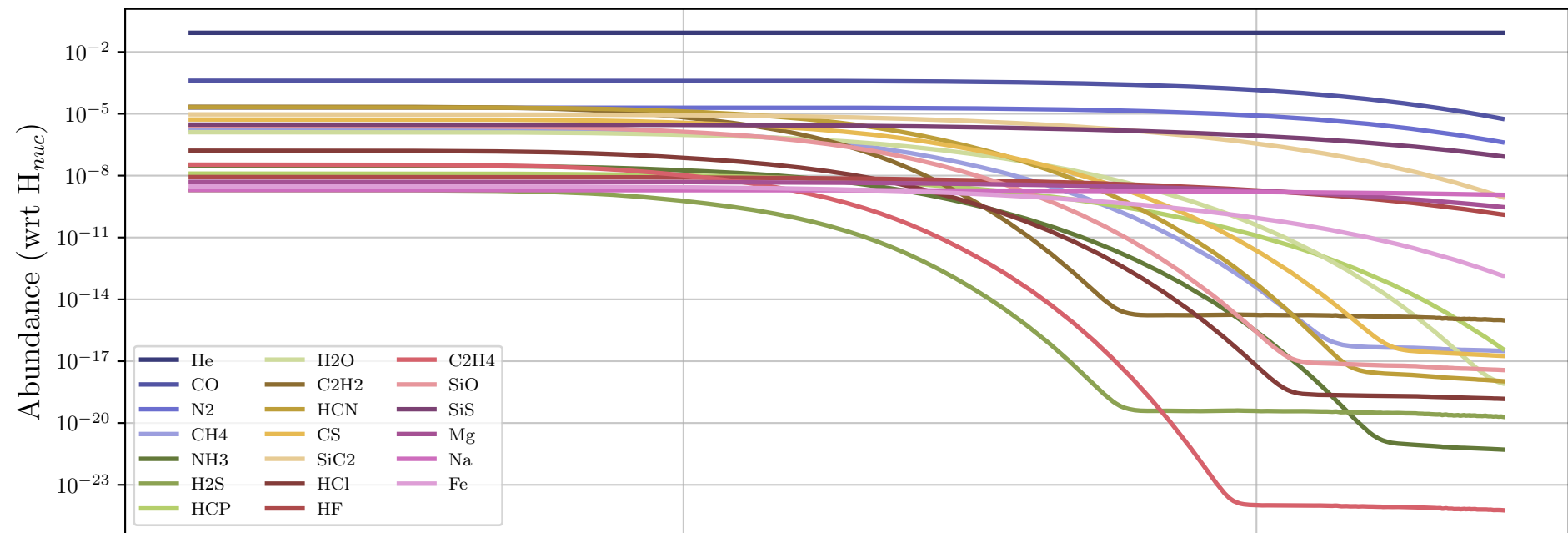
Particle 107695 - Parent Molecules
