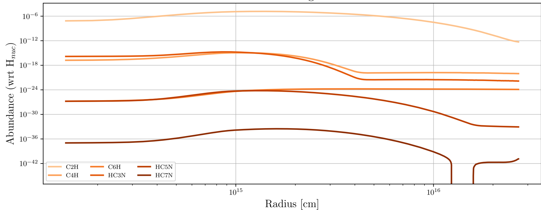
Particle 107695 - Daughter Molecules
